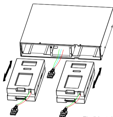
Fig.5 Installation for battery pack
