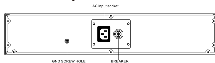
Fig.7 Battery pack rear panel
