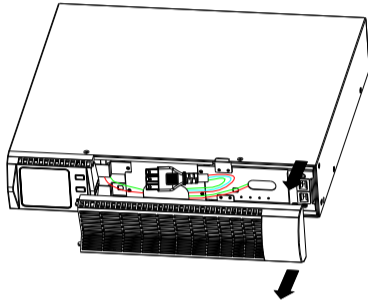
Figure1 Removing the EBP Front Cover
