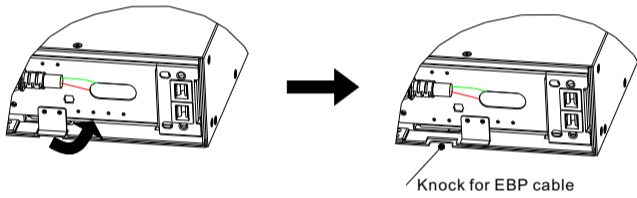
Figure2 Removing the UPS and EBP Cable Knockout
